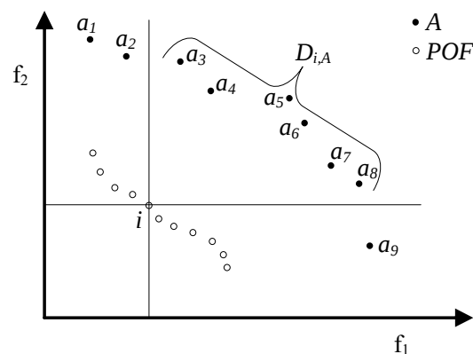
Figure 8. D_{i,A} of a point i belonging to the POF (example with n = 2 ).
