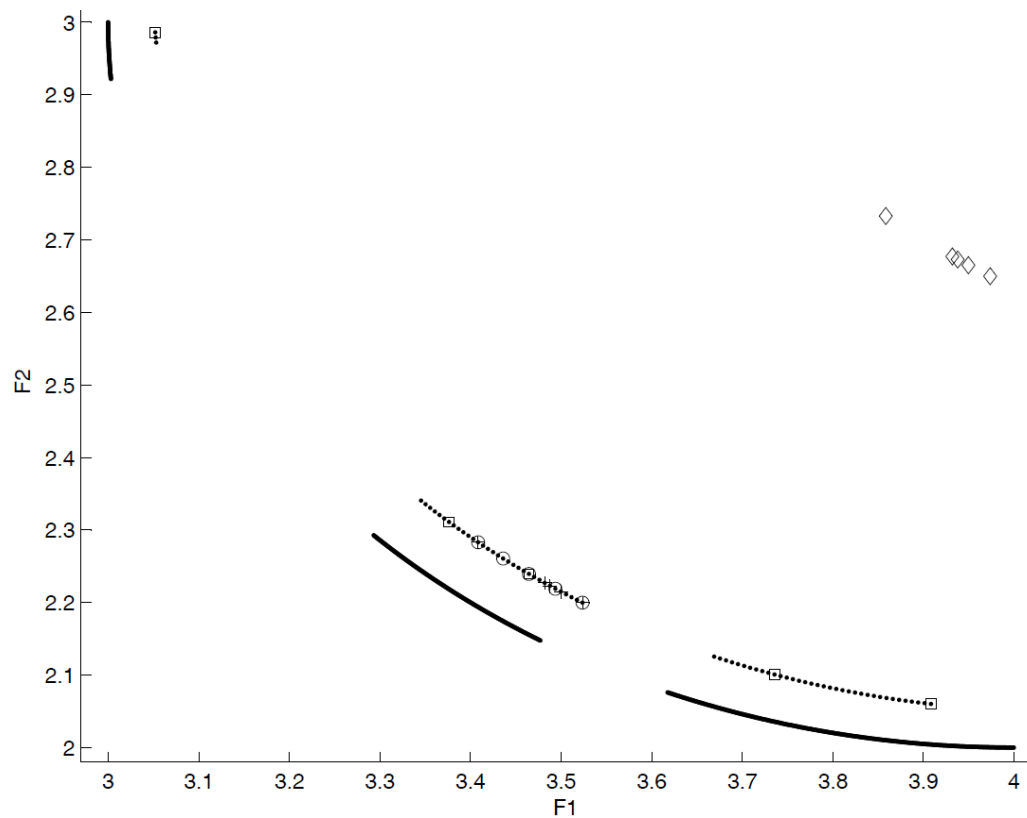
Figure 16. Convex and disconnected POF (solid line), APF1 ( \diamond ), APF2 (+), APF3 ( \circ ), APF4 ( \square ) and APF5 ( \bullet ).
