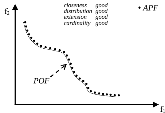
Figure 7. An APF with all the desired features.
