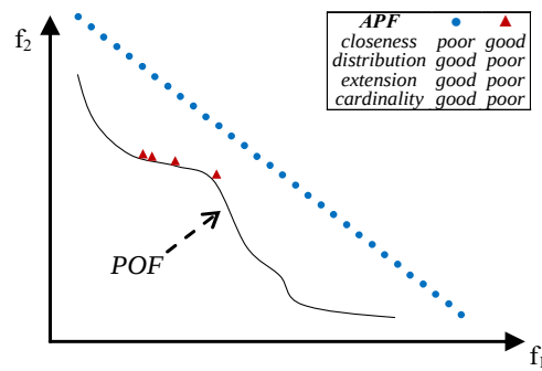
Figure 3. An APF (blue dots) with all good features but not close to the POF and another (red triangles) that is only close to the POF.
