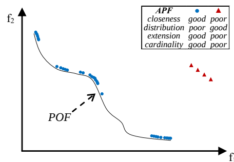
Figure 4. An APF (blue dots) with all good features but not uniformly distributed and another (red triangles) that is only uniformly distributed.
