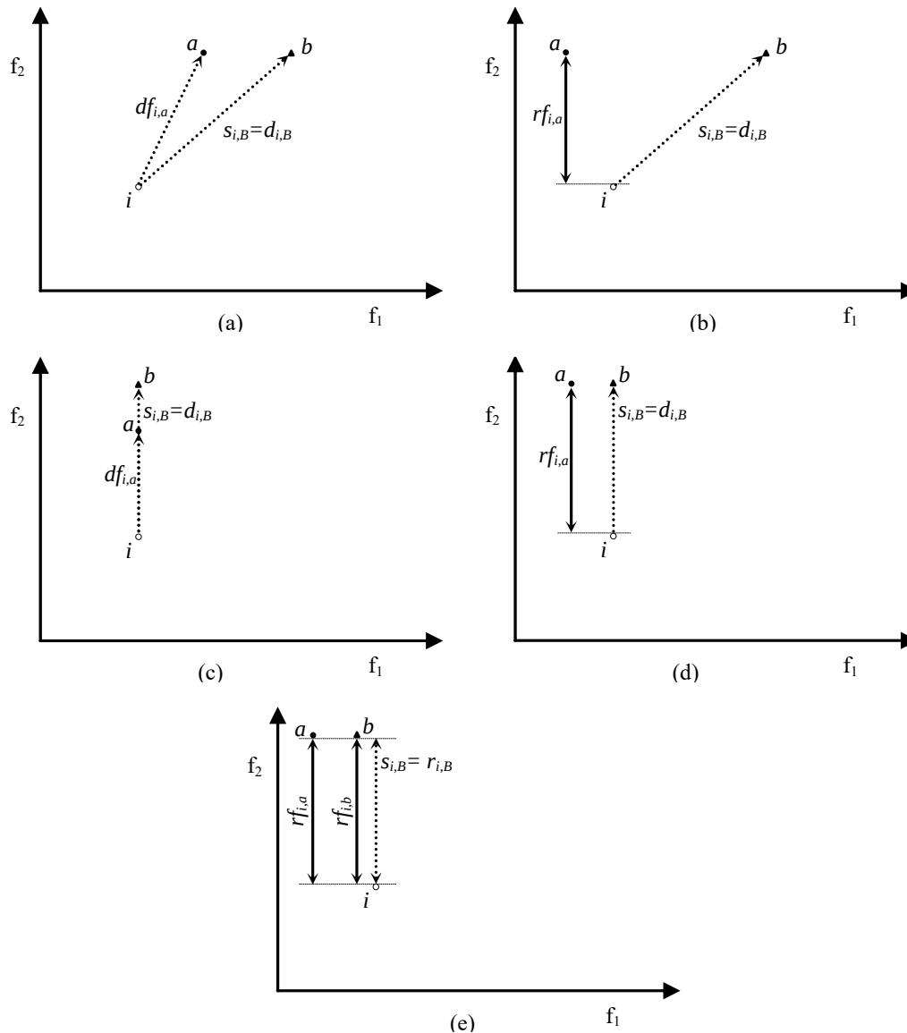
Figure 13. Possible scenarios for A \succ B . (a) scenario A2 or C2; (b) scenario B2 or D2; (c) scenario C2: limit case; (d) scenario D2: limit case; (e) scenario E2.
