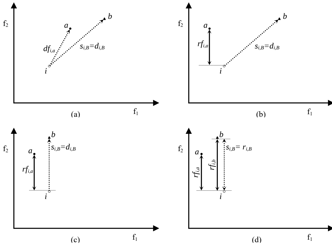
Figure 12. Possible scenarios for A \succ \succ B . (a) scenario A1: most relevant case; (b) scenario B1 or C1; (c) scenario C1: limit case; (d) scenario D1.
