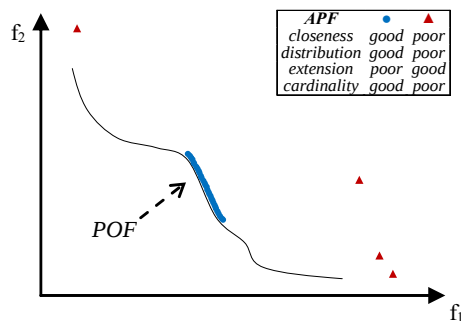
Figure 5. An APF (blue dots) with all good features but not extended and another (red triangles) that is only extended.
