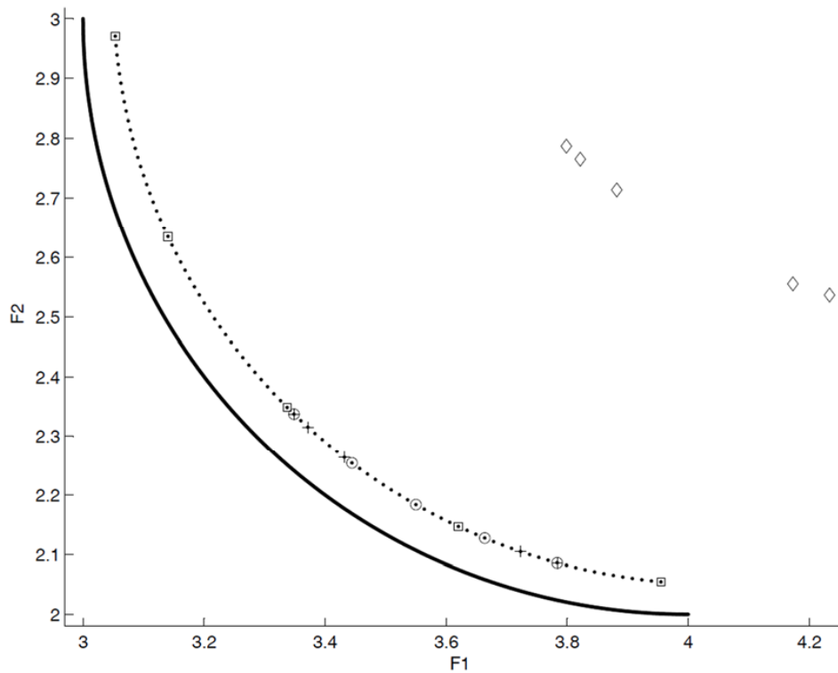
Figure 14. Convex and connected POF (solid line), APF1 ( \diamond ), APF2 (+), APF3 ( \circ ), APF4 ( \square ) and APF5 ( \bullet ).
