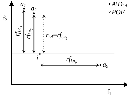
Figure 10. r_{i,A} of a point i belonging to the POF.
