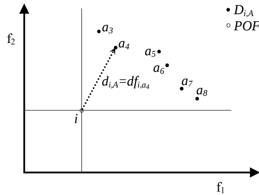
Figure 9. d_{i,A} of a point i belonging to the POF.
