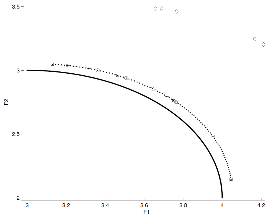
Figure 15. Non-convex and connected POF (solid line), APF1 ( \diamond ), APF2 (+), APF3 ( \circ ), APF4 ( \square ) and APF5 ( \bullet ).
