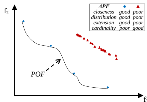
Figure 6. An APF (blue dots) with all good features but with poor cardinality and another (red triangles) that has only high cardinality.
