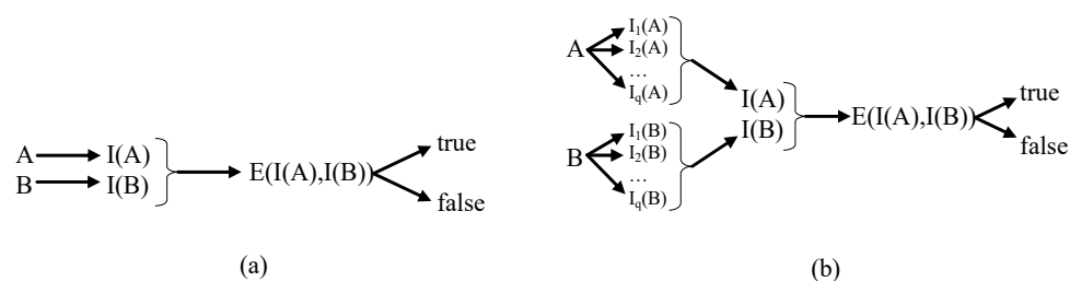
Figure 2. Comparison method in case of one QI (a) and in case of a vector of q QIs (b).
