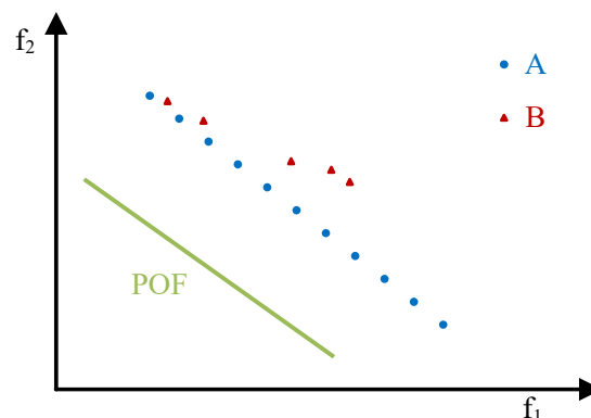
Figure 1. In this case A and B are incomparable in terms of Pareto dominance, but A is preferable to B because A is closer to the Pareto-optimal front (POF), more extended, more populated, and better distributed.
